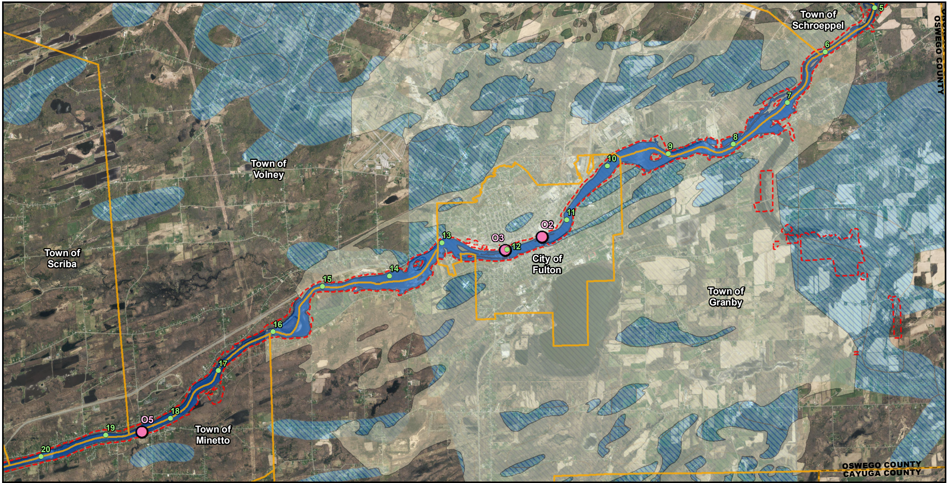
Figure 68F: Aquifers
